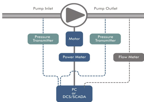
Ultrasonic Pump Test Arrangement
