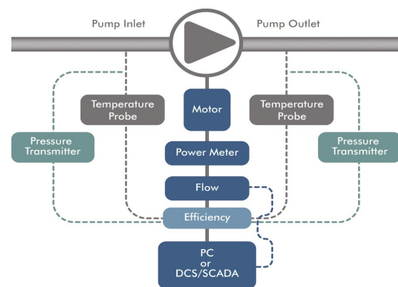
Thermodynamic Pump Test Arrangement
